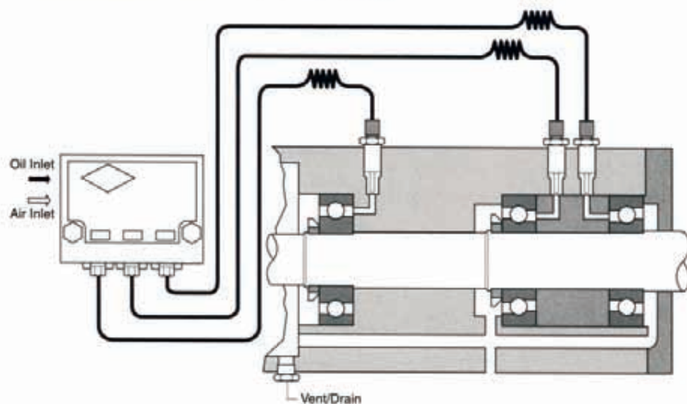
Typical high-speed spindle installation.
