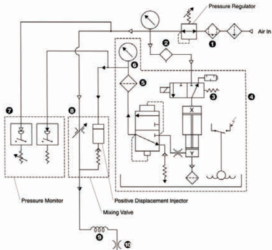
Schematic of the HyperFormance system with components identified at left.
